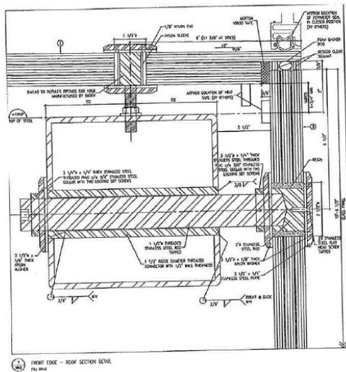
Figure 4: Glass Panel Hanging Detail
