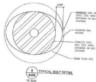
Figure 8: Typical Bolt / Oval Bushing Detail
