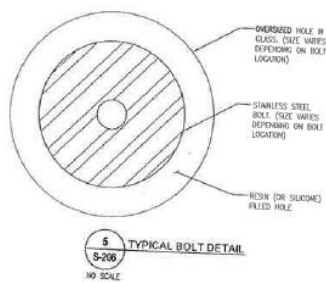
Figure 7: Typical Bolt Detail
