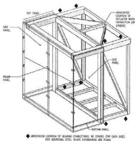
Figure 2: Isometric view of Steel Frame and Glass
